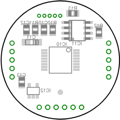
Figure 6 Solder Side
