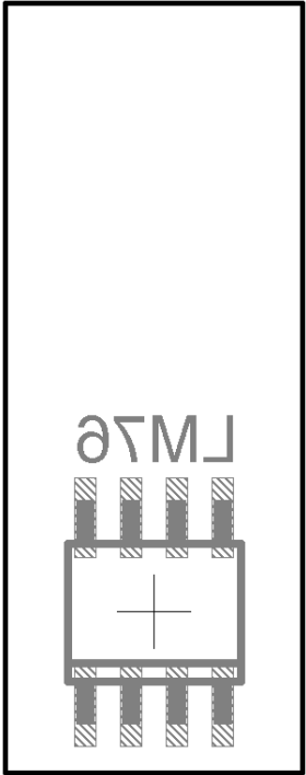
Figure 3 Solder Side
