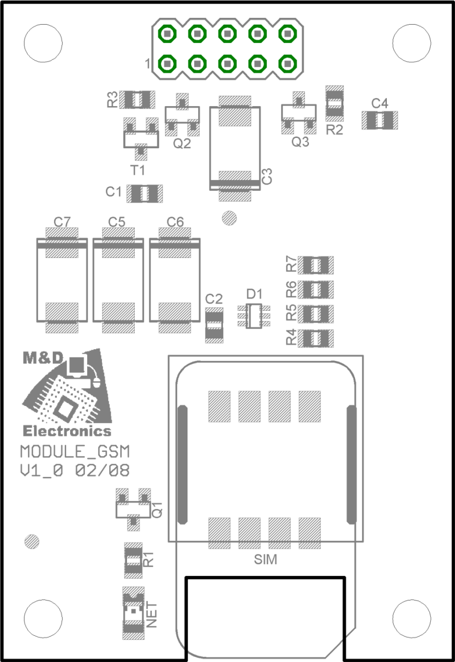
Figure 1 Component Side
