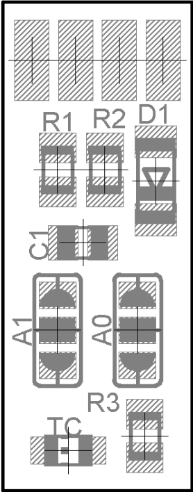
Figure 4 Component Side
