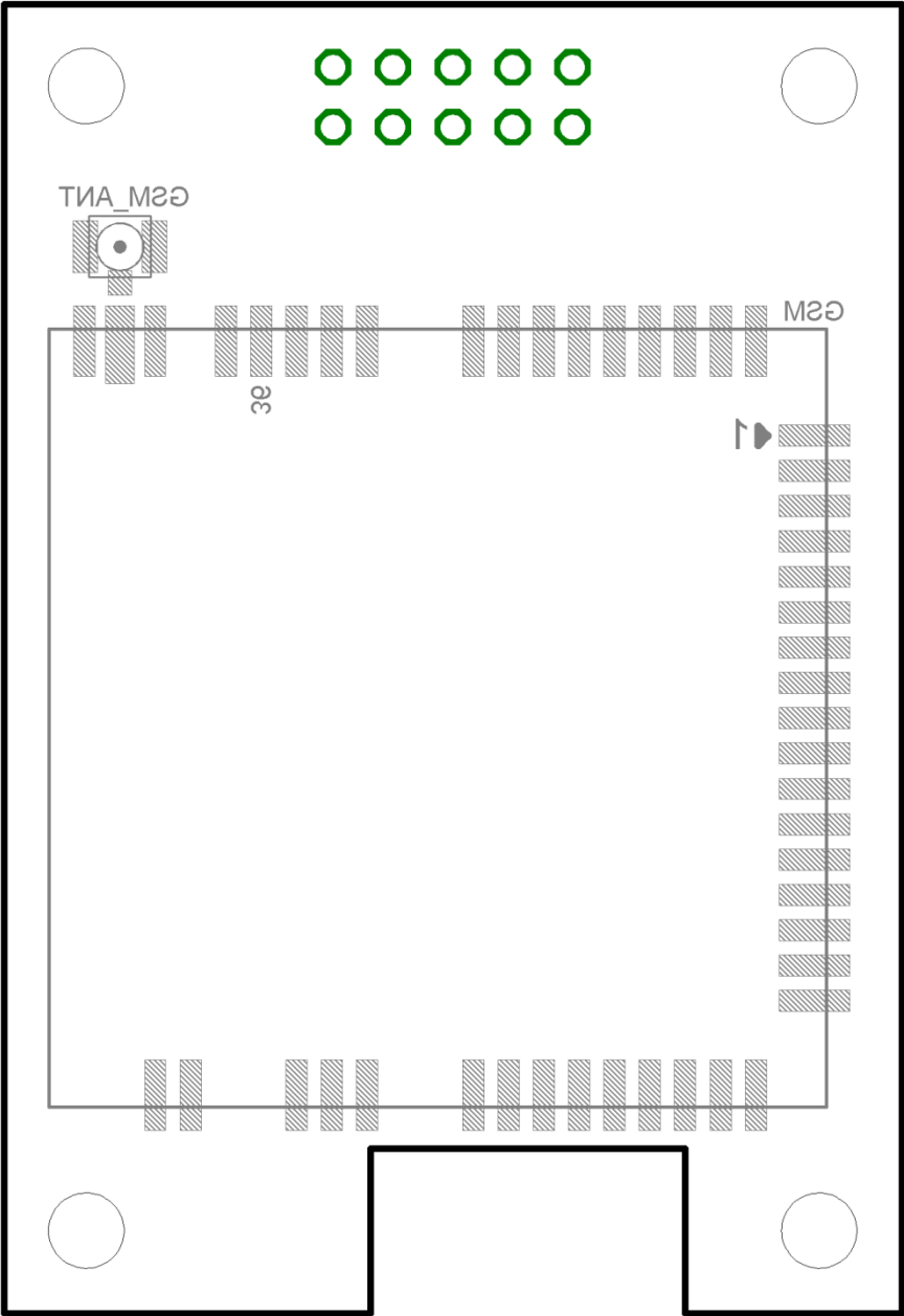
Figure 2 Solder Side
