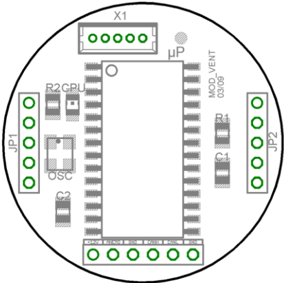
Figure 5 Component Side
